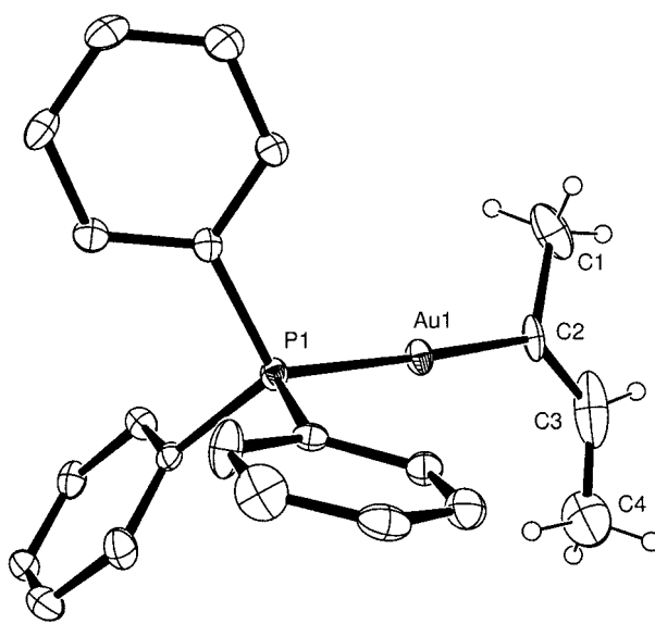
Figure 1. ORTEP view of one of the independent molecules of 6a . Ellipsoids show 30% probability levels; phenyl hydrogen atoms have been omitted for clarity.
